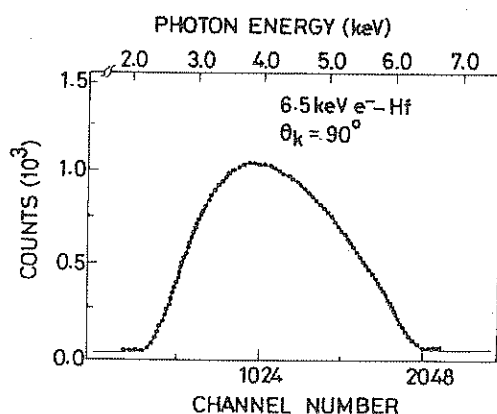
Figure 1. A typical bremsstrahlung X-ray photon energy spectrum produced in 6.5 keV e^- -Hf collisions. Photons are detected at \theta_k = 90^\circ with respect to the incident electron beam direction.
