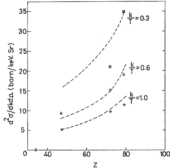
Figure 4. Variation of the absolute doubly differential cross-sections, d^2\sigma/dk d\Omega (barn/keV.sr) as a function of atomic number Z of the targets; Ag, Hf and Au for k/T = 0.3 (■), 0.6 (▲) and 1.0 (●) in 7.0 keV e^- -Ag, Au and 7.5 keV e^- -Hf collisions. Dotted curves represent the theoretical predictions [8]. Error bars (not shown) are similar to ones shown in figures 2 and 3.
