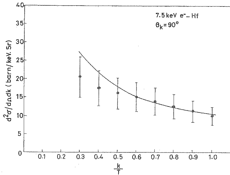
Figure 3. Same as in figure 2 except for 7.5 keV electrons incident on Hf target (filled circles).
