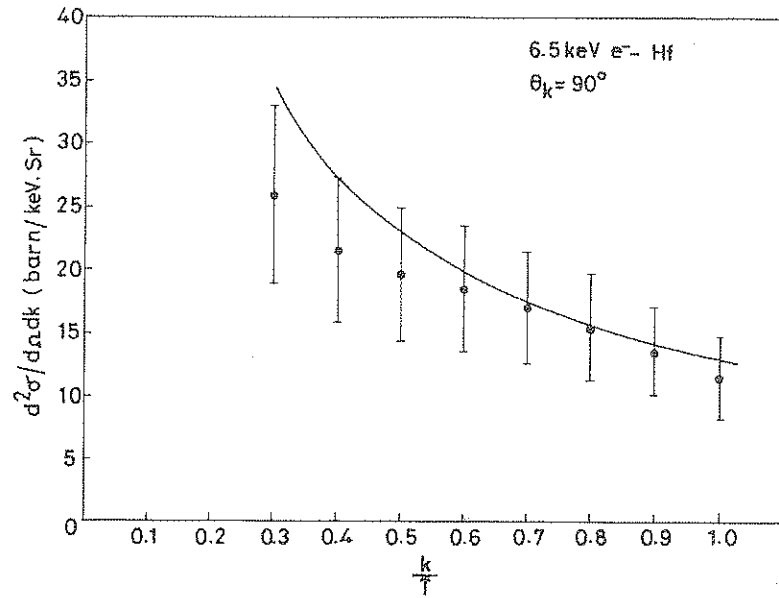
Figure 2. Absolute doubly differential cross-sections, d^2\sigma/dk d\Omega (barn/keV.sr) for bremsstrahlung photons emitted from 6.5 keV electrons colliding with a Hf target (filled circles), as a function of the photon energy radiated per incident electron energy, k/T . The solid line curve is theory [8]. Error bars represent the systematic error of measurements.
